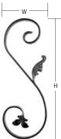
BS-662 - 1/4" x 1/2" 7"W x 19"H
