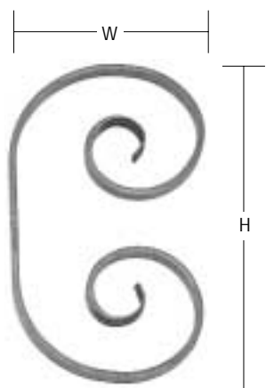
S-206 — 1/4" x 1/2" 6-1/2"W x 13"H
