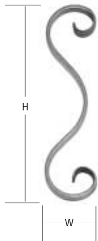
FS-406 — 1/4" x 1/2" 3-1/4"W x 13"H
