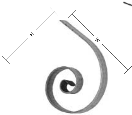
HE-2000 — 1/4" x 1-1/2" 12"H x 13-1/4"W
